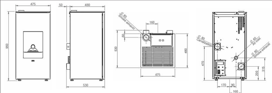
SAEY QUBIC 10 (TWIN)
