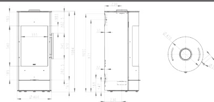
SAEY CURVE EVO
