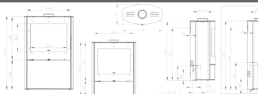
SAEY FURA EVO / HIGH
