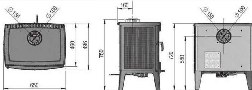
SAEY PEAK GAS
